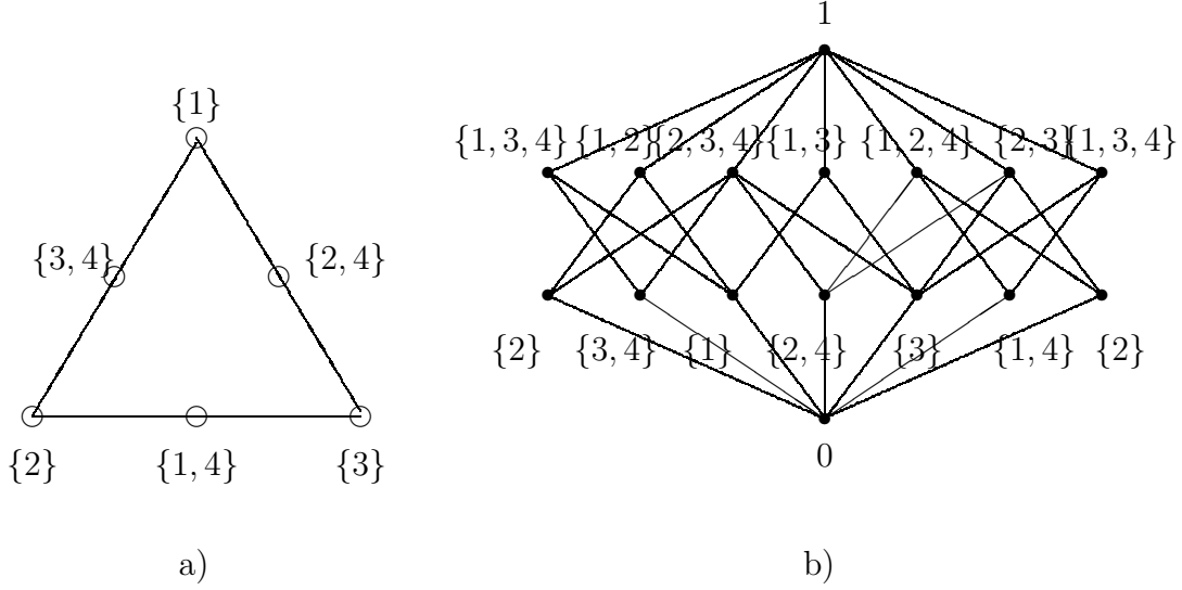
Fig. 2. a) Greechie and b) Hasse diagram of a logic featuring complementarity which is not a quantum logic but which is embeddable in a Boolean logic.
